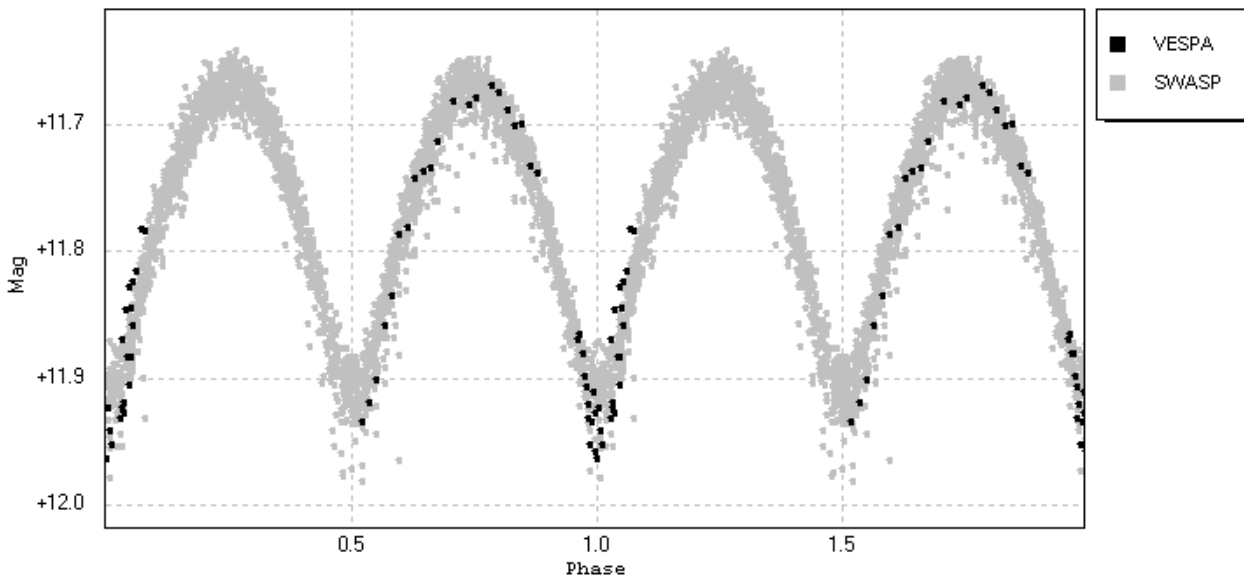
VESPA_V19 - P= 0.401534 - E= 2456963.48117
